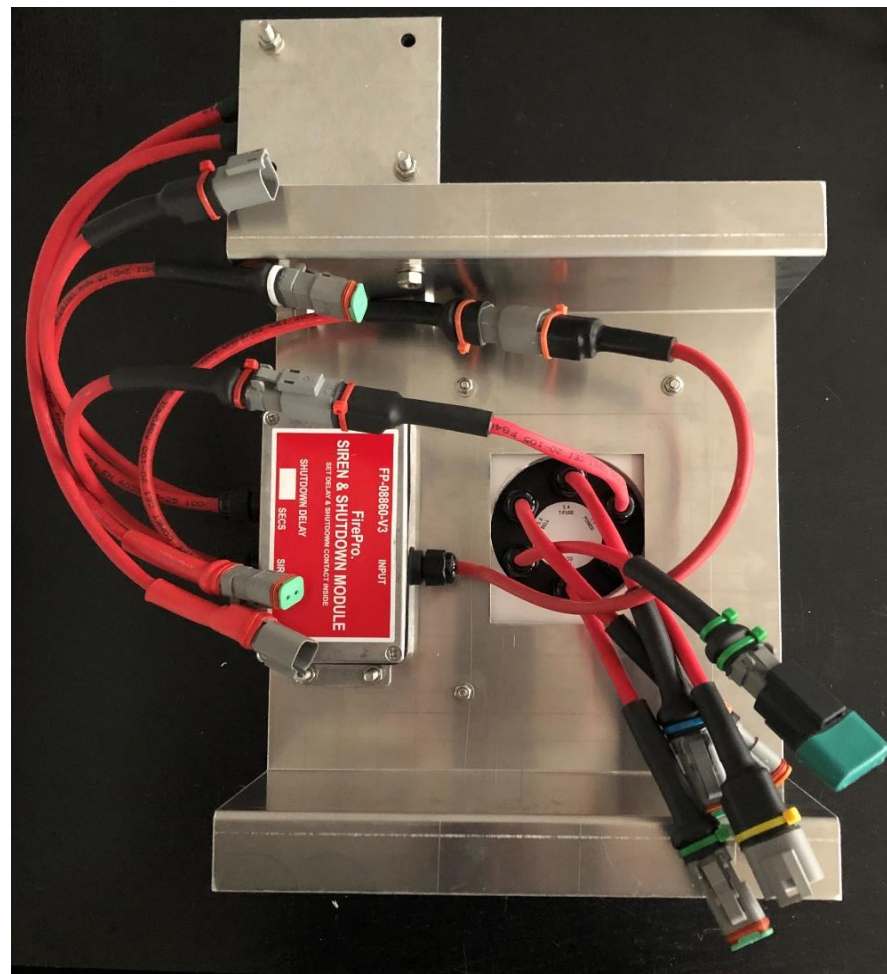
REAR MOUNTED VIEW
