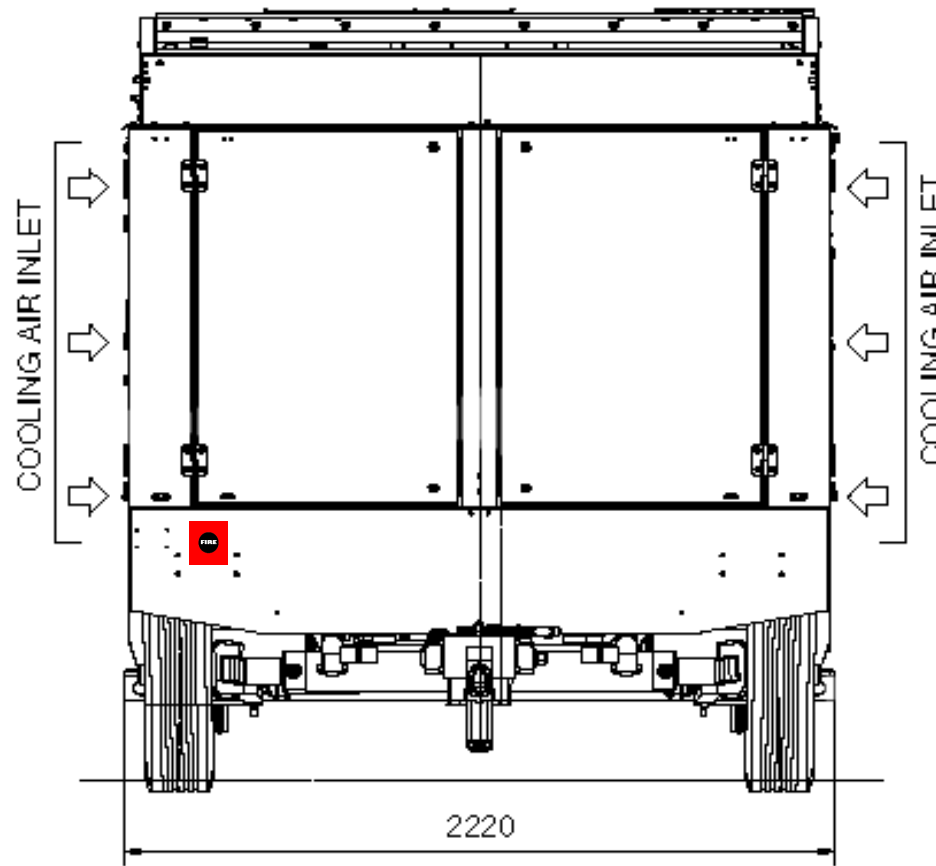
FRONT MOUNTED VIEW
