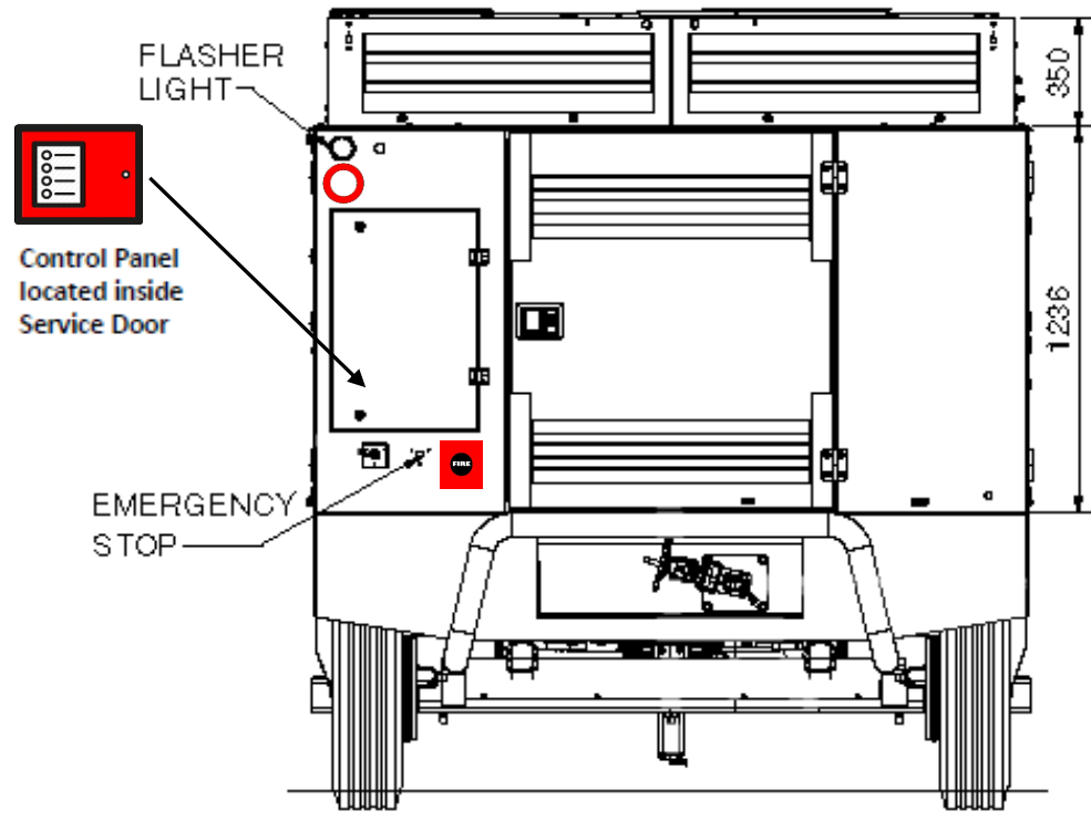
REAR MOUNTED VIEW
